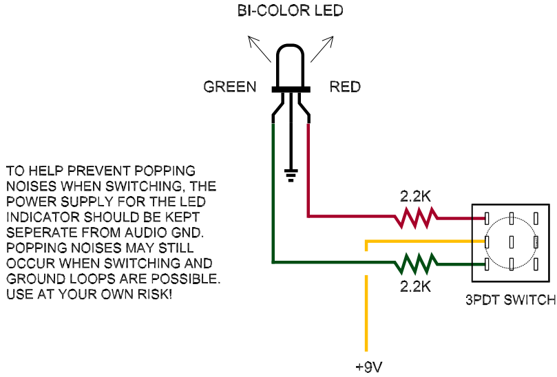
LED INDICATOR SECTION
