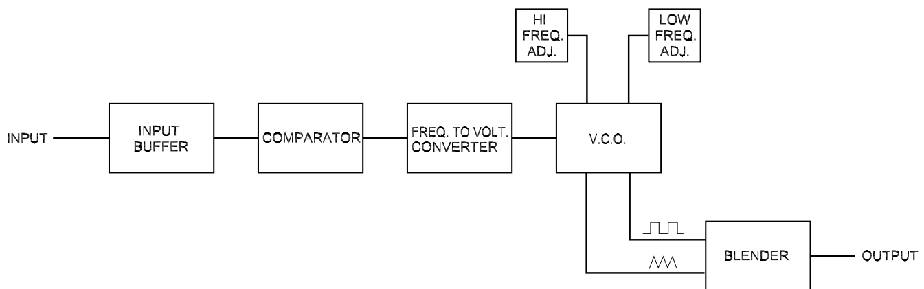
GUITAR-SYNTH-IN-A-BOX BLOCK DIAGRAM
