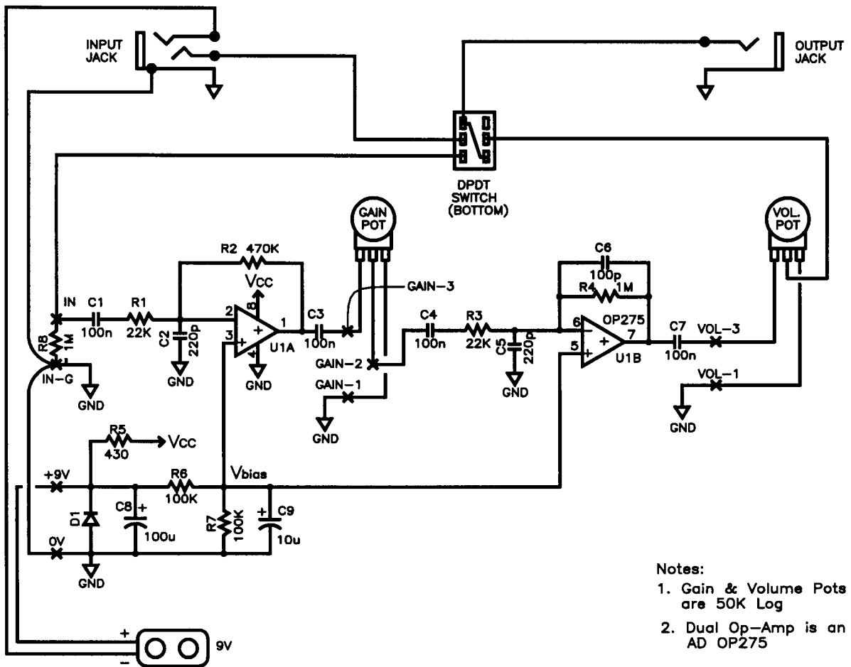
Black Cat OD-1 Schematic
