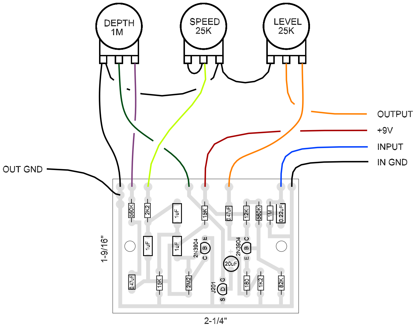
EA Tremolo Layout by Paul Marossy 10/25/03
