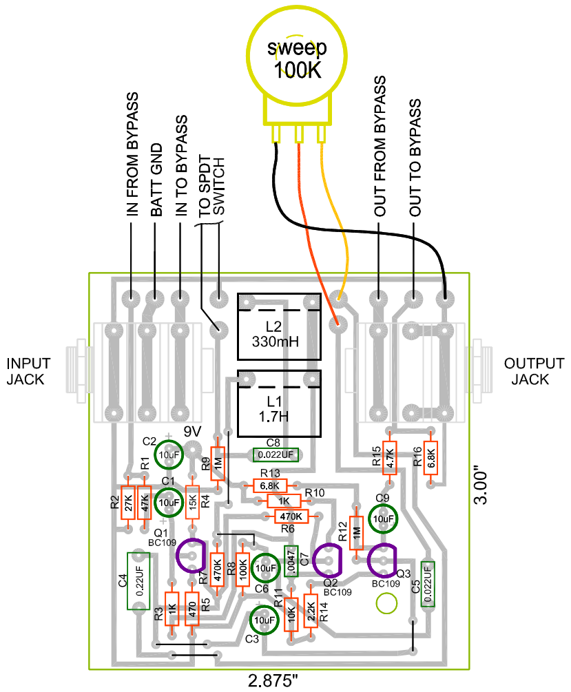
SCHALLER "BOW WOW YO YO YO" PCB LAYOUT BY PAUL MAROSSY 2/25/13
