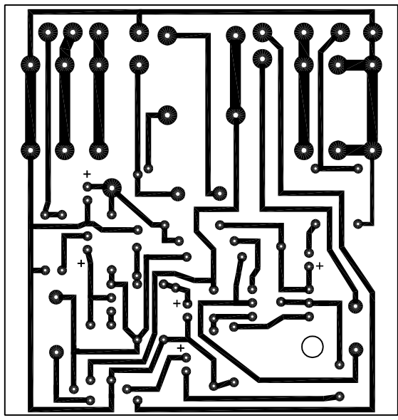
SCHALLER "BOW WOW YO YO YO" PCB LAYOUT BY PAUL MAROSSY 2/25/13
